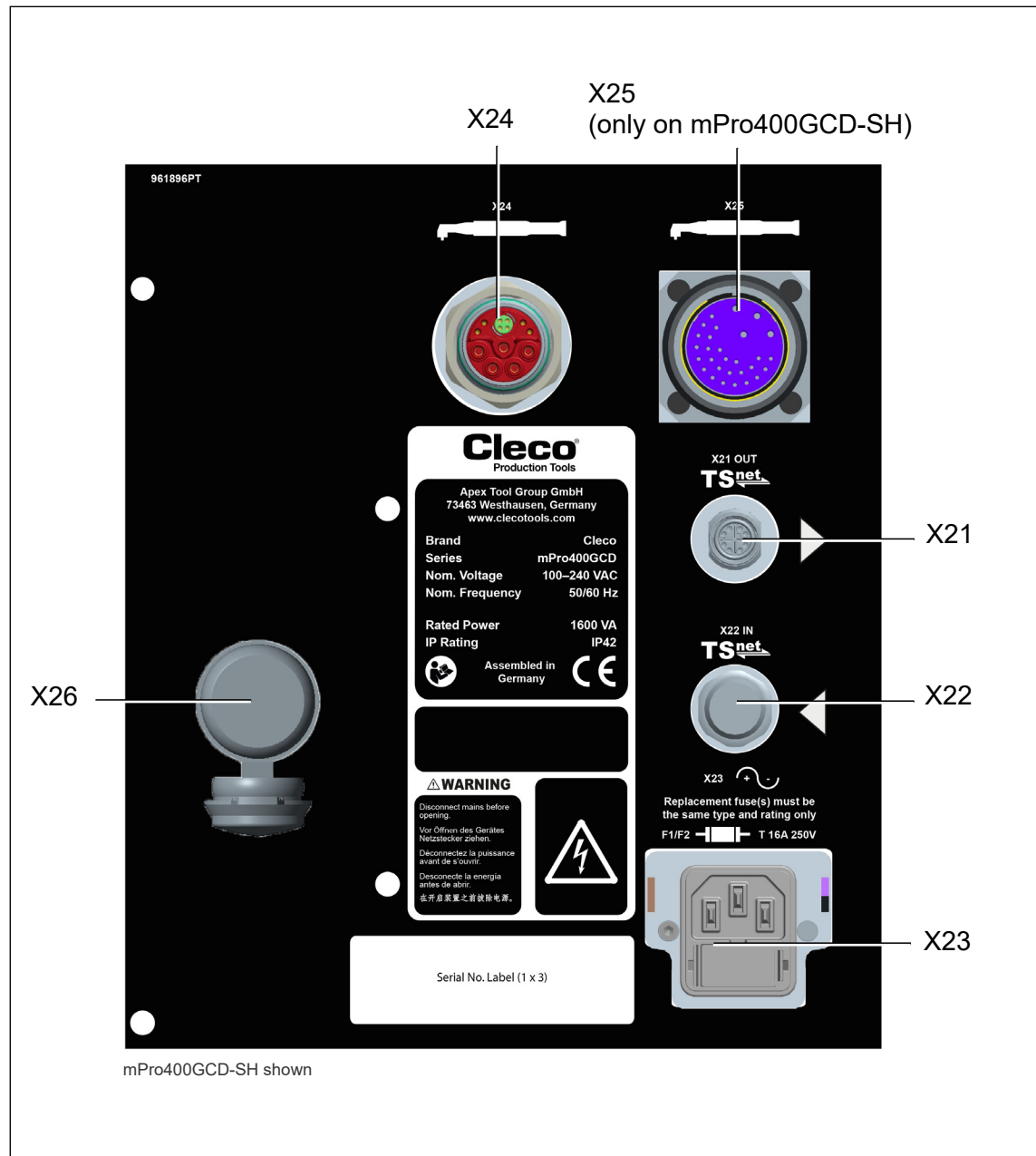
Abb. 8-1: Connection positions
